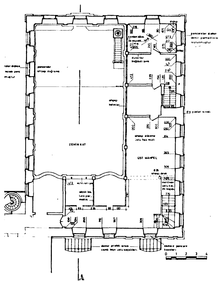
BİRİNCİ KAT PLANI 1/100
