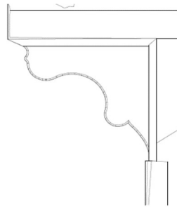
47.p- Kıvrımlı ahşap payandalar 0 10 20 30 40 50 cm
