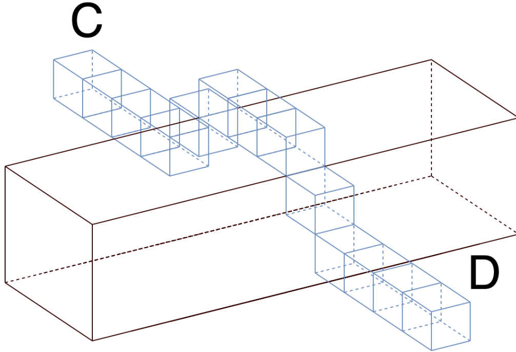
Figure 4.7 A path planned from C to D considering previously inflated active path
