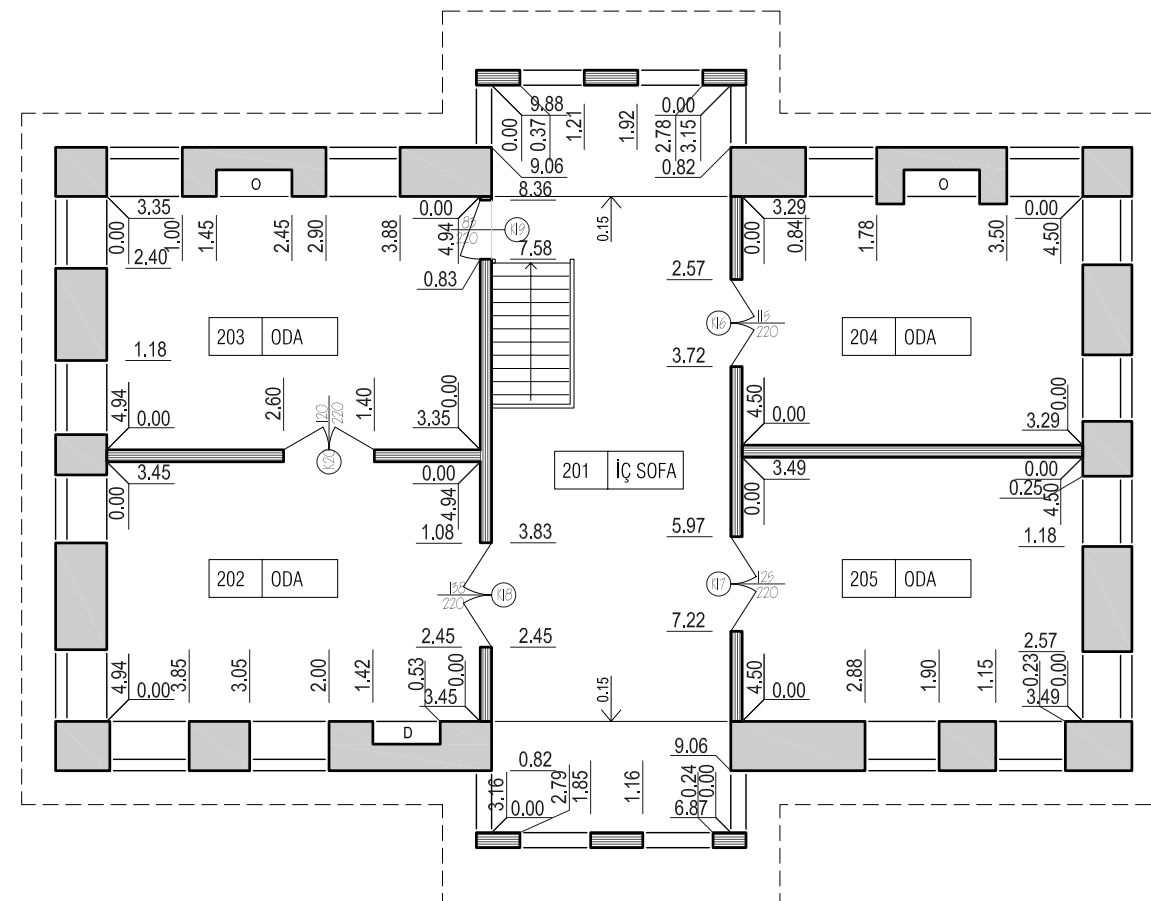
2. KAT PLANI
